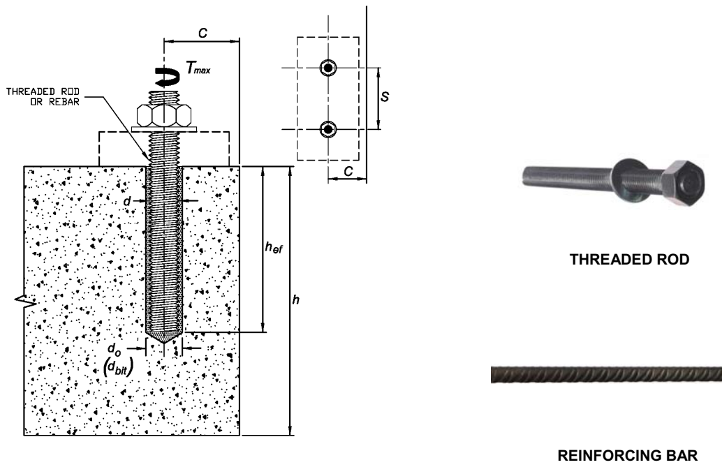
FIGURE 2—INSTALLATION PARAMETERS FOR THREADED RODS AND REINFORCING BARS
